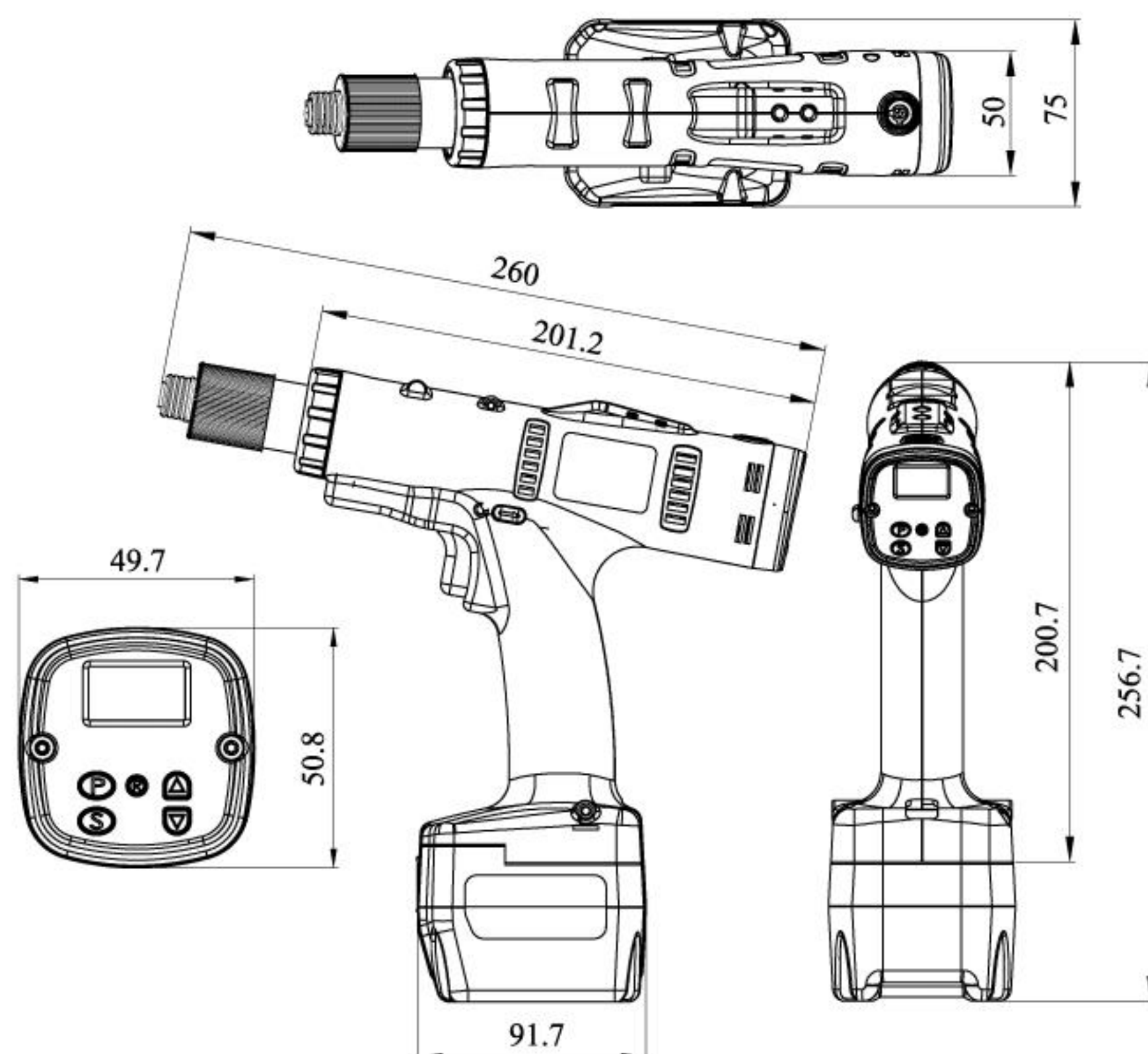
MYBT-EP0612 Unit: mm
